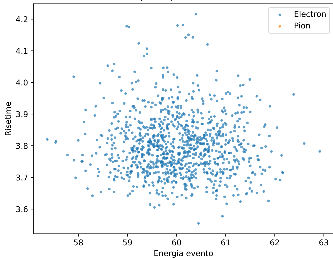
Scatter plot e/pi (cutted) 60.0GeV
