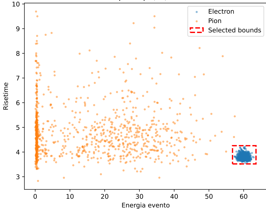
Scatter plot e/pi (all) 60.0GeV
